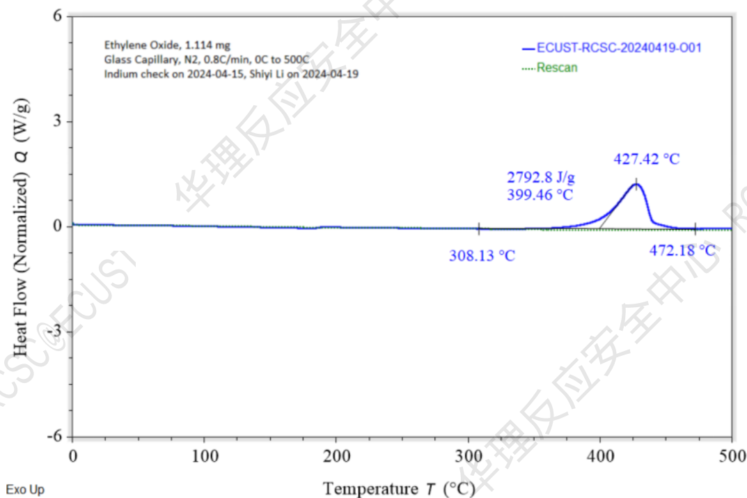
Figure 2. DSC Curve with -6~6 W/g scale, the solid line represents the first scan (with integration); The dashed line represents the second scan
